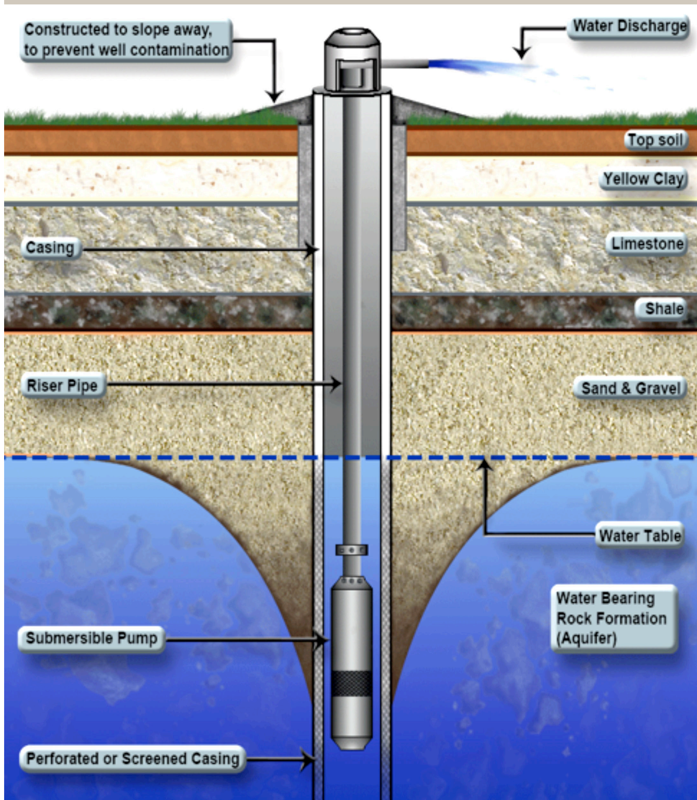
Typical well diagram
